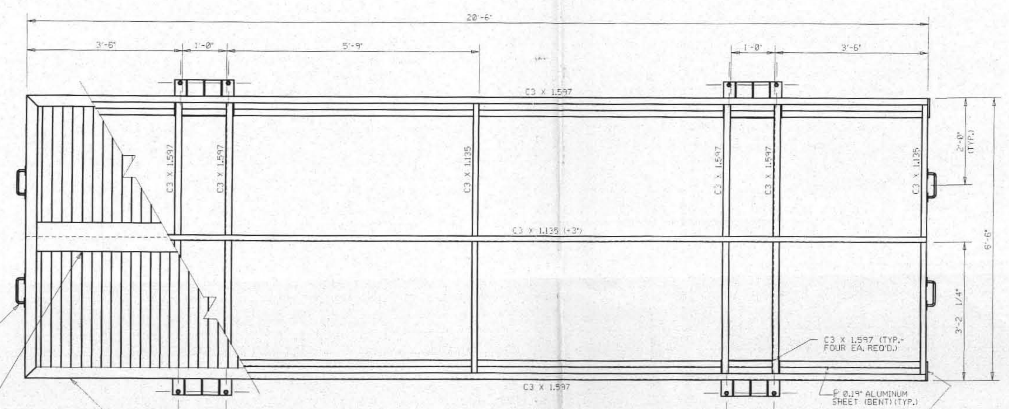
PORTABLE COVER (PLAN VIEW) SCALE: 3/4" = 1'-0"
