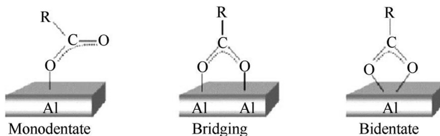
Fig. 9. Proposed carboxylate binding to aluminum surface in acid coating of aluminum powders [50].
